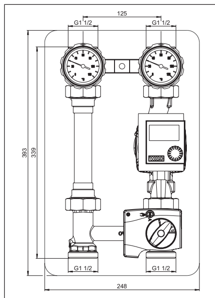
Illustr. 6 Boiler connection system with three-way mixing valve 180 mm DN25 with pump ball valve (short version)
