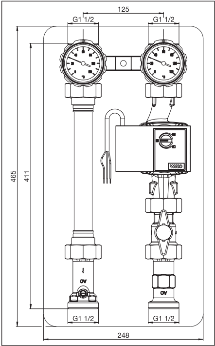
Illustr. 3 Boiler connection system 180 mm DN 25 with pump ball valve (long version)
