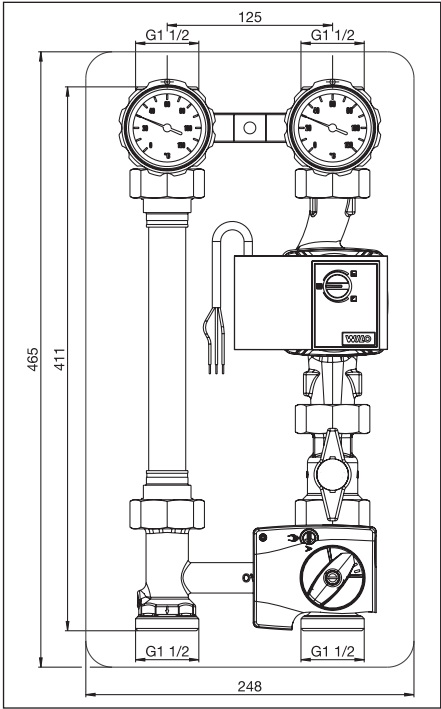
Illustr. 4 Boiler connection system with three-way mixing valve 180 mm DN 25 with pump ball valve (long version)
