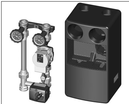
Illustr. 1.1 Boiler connection system with 3-way mixing valve (Depending on the model, supplied with or without ventilation grille).
