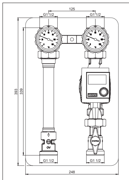
Illustr. 5 Boiler connection system 180 mm DN25 with pump ball valve (short version)
